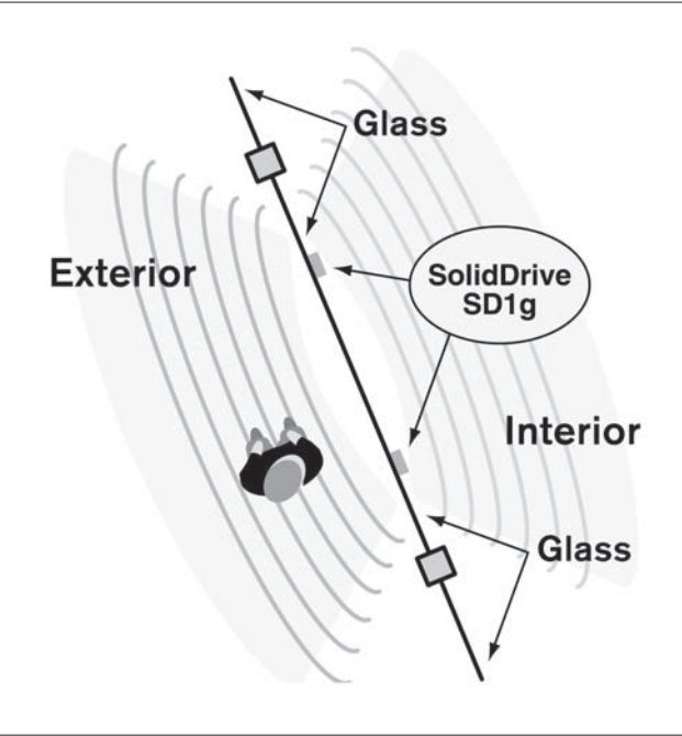
Figure 4 How the SolidDrive SD1g works on glass
