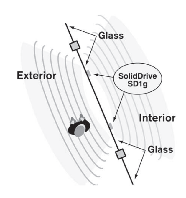
Figure 4 How the SolidDrive SD1g works on glass
