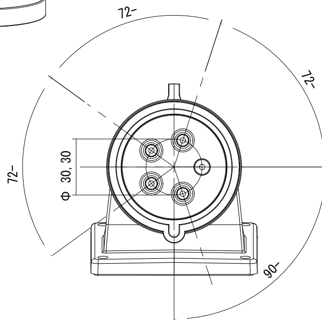
Type 77725-9/ Flanged plug angled 32A 5p 9h IP44
