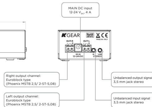
GA201 Front Panel
