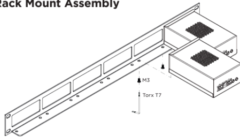
Rack Mount Assembly
