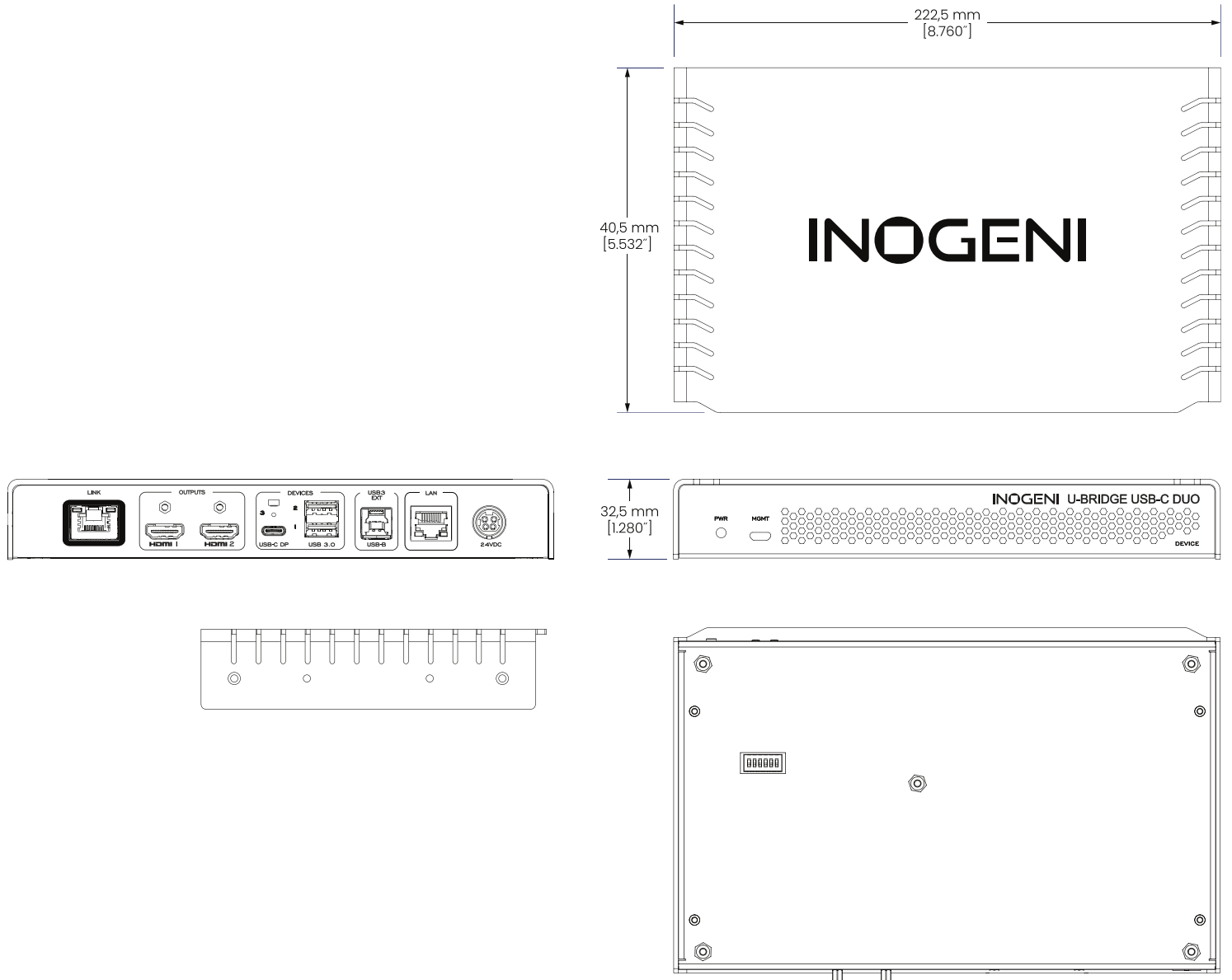
Figure 4: Bottom plate dimensions and holes positions of DEVICE hub – DUO variant
