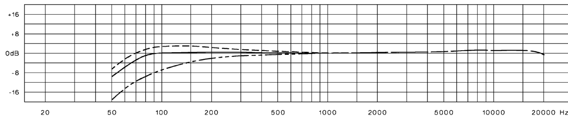
Frequency response ±2.5 dB 0 dB = 14 mv/Pa MPC 67
