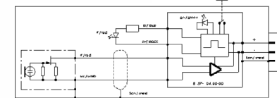
Classis GM 314 S - 315 S
