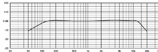
Frequency response curve ± 2.5 dB 0 dB ≙ 17 mV/Pa Classis GM 314 - 315
